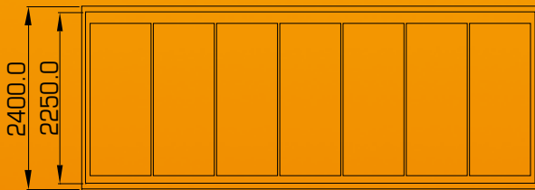
CONTAINER 20" - 7 PALLETS
